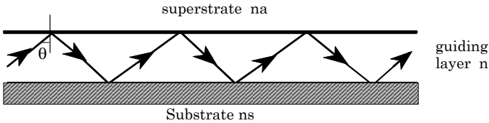
Figure 1.6. Guided modes
