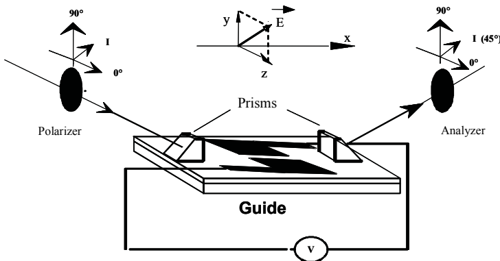
Figure 5.11. Polarimetric setup
