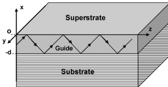
Figure 1.1. Planar optical waveguide
