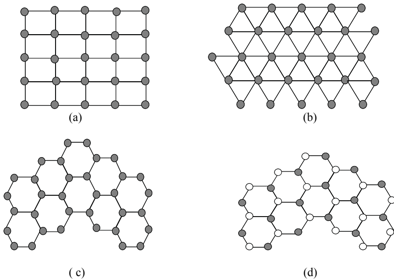
Figure 6.8. Examples of 2D photonic crystal cells
