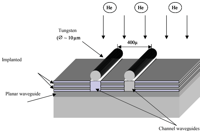
Figure 2.15. Creation of a channel optical waveguide using multiple implantation through a tungsten micro wire mask
