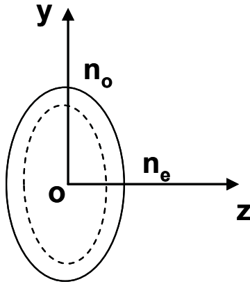
Figure 5.4. Meridian section of the index ellipsoid with and without the electric field E parallel to the optical axis
